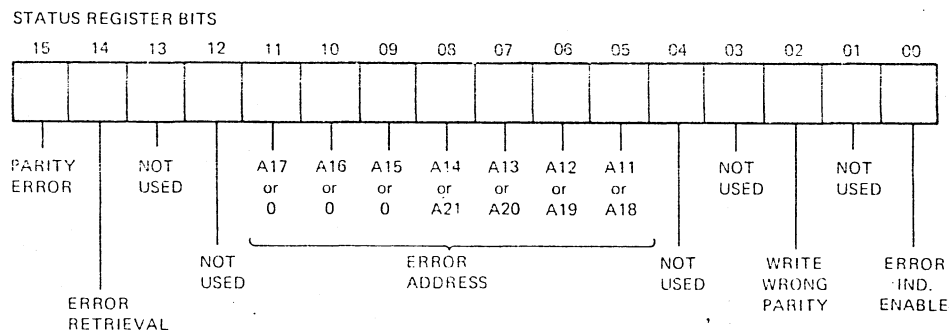
Figure 2-4 CSR Bit Allocation
